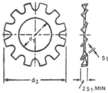
Type A: Externally Toothed T
