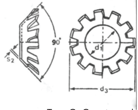
Type C: Countersunk
