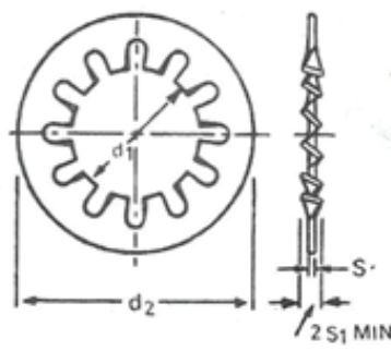
Type B: Internally Toothed
